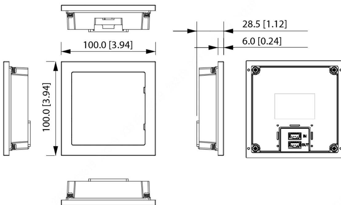
Figure 3-1 Dimensions (unit: mm [inch])
