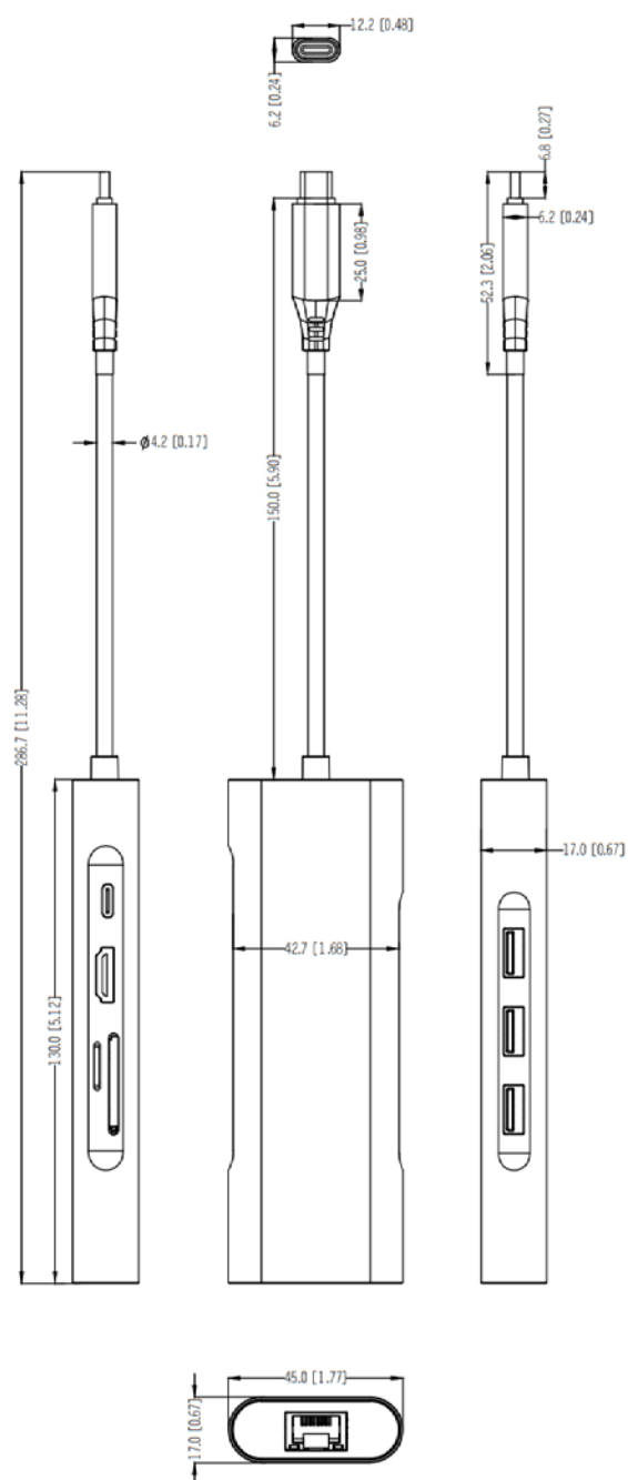
Figure 1-1 Dimensions (Unit: mm [inch])
