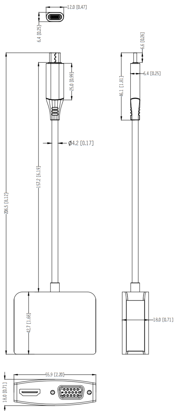
Figure 1-1 Dimensions (Unit: mm [inch])
