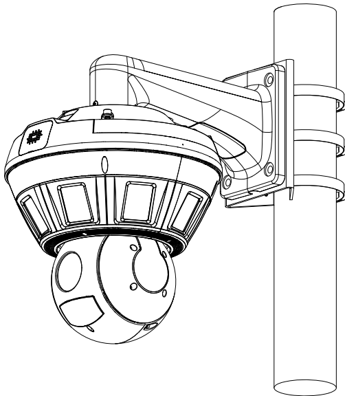
Pole Mount(Vertical)
