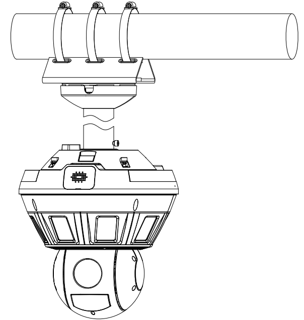
Pole Mount(Horizontal)
