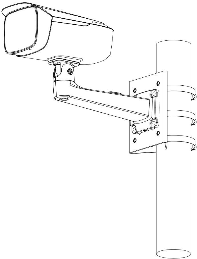
Pole Mount(Vertical)
