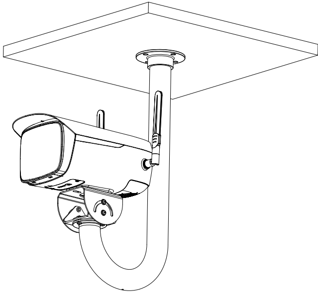
Ceiling Mount
