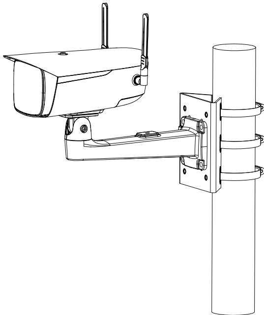
Pole Mount(Vertical)
