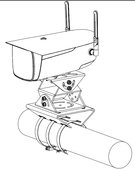
Pole Mount(Horizontal)
