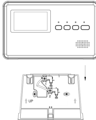
Figure 3-6 Installation (4)
