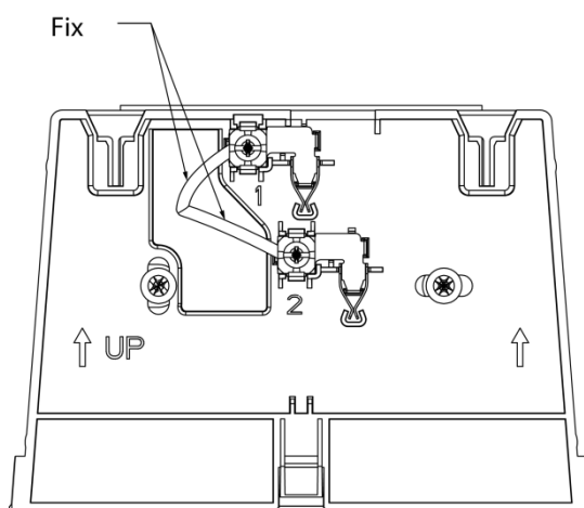
Figure 3-3 Installation (2)
