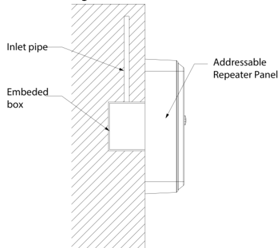
Figure 3-6 Installation (4)
