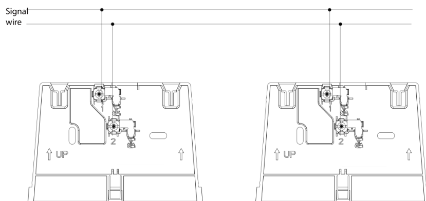
Figure 3-3 Installation (2)
