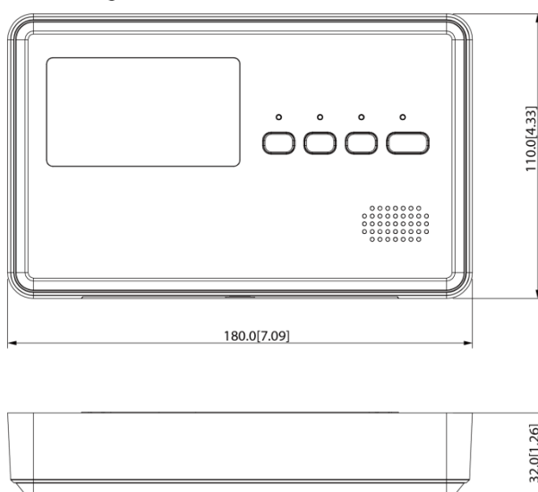
Figure 1-1 Dimensions (mm[inch])
