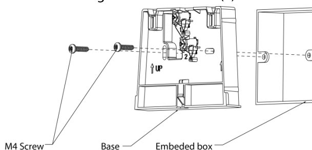
Figure 3-1 Installation (1)
