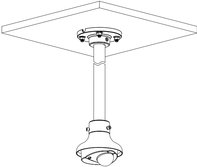
Ceiling Mount
