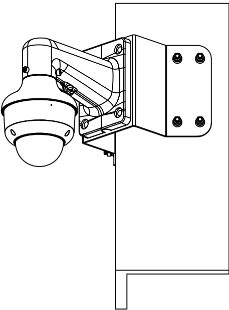
Corner Mount
