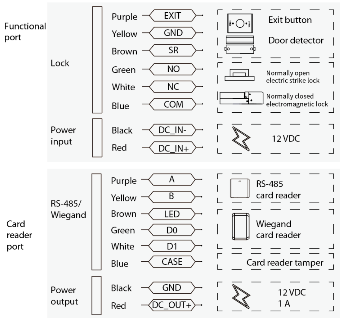
Figure 2-4 Cables
